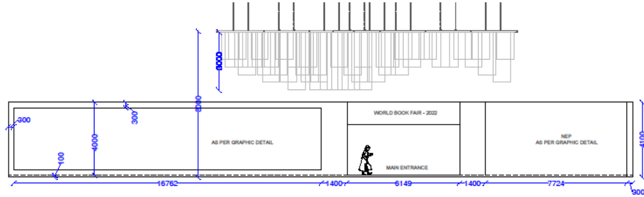
ELEVATION-B
