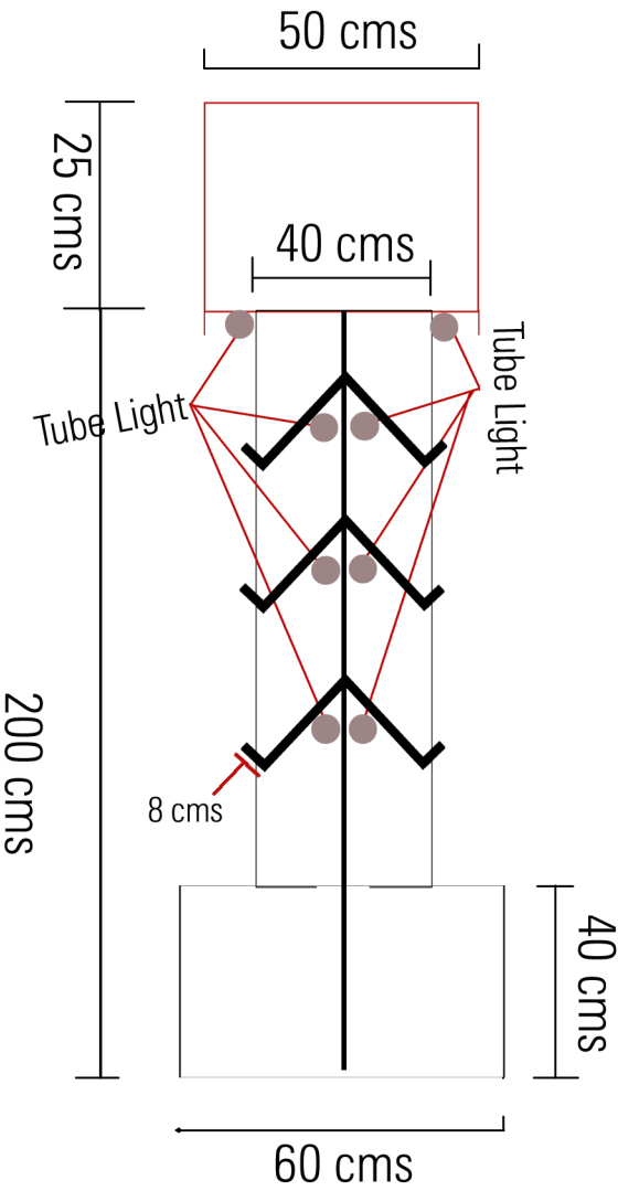
Side Elevation
