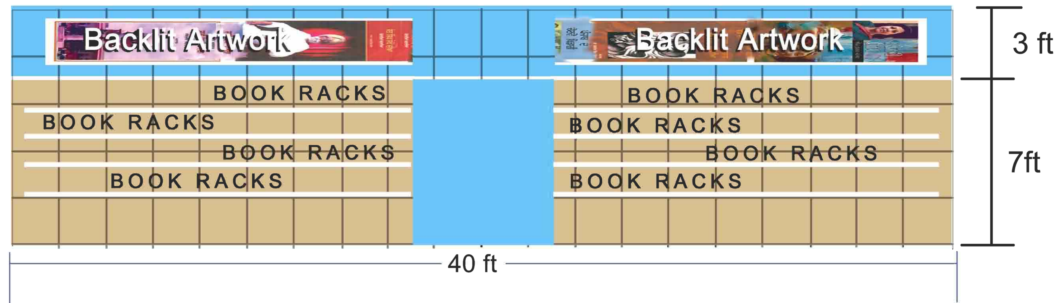
Floor plan (40X20)
