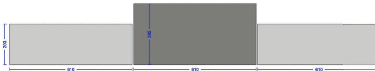
Front Elevation
